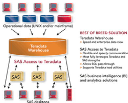
Figure 1. typical SAS / DB architecture
